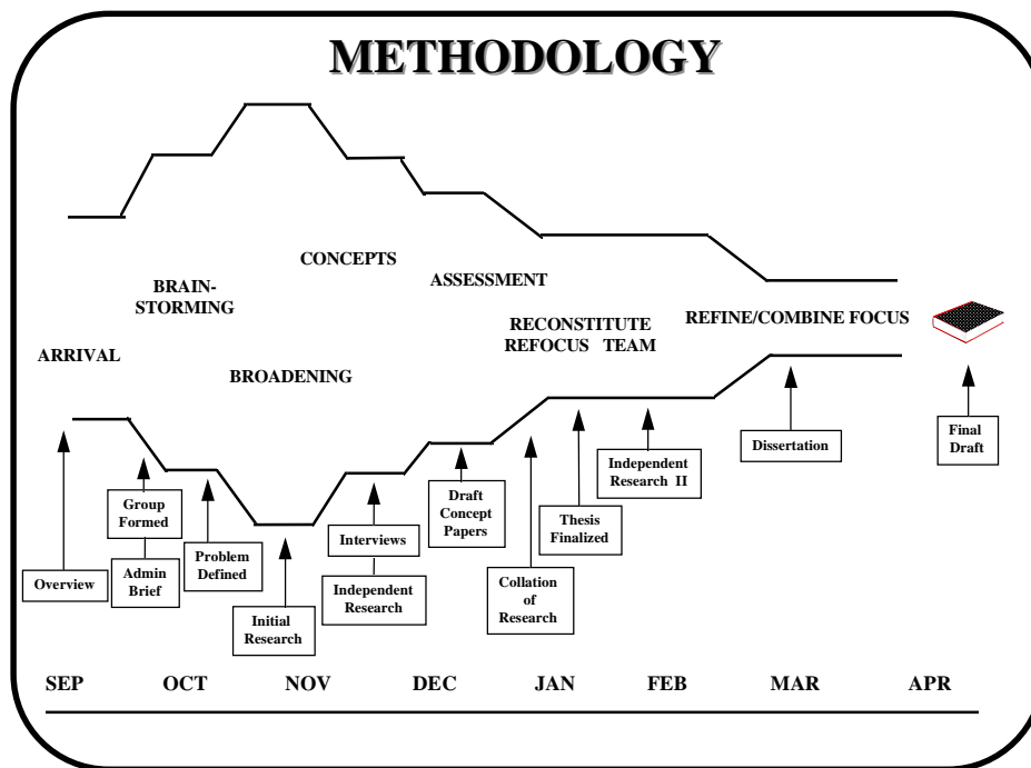
Figure 4. Methodology
