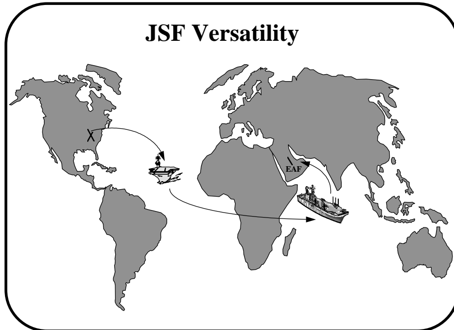
Figure 10. JSF Versatility
